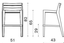
Counter stool h82 RBSGH1T1 cushion RBCUSGA_
