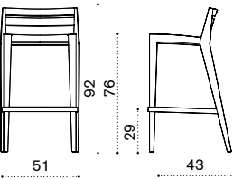
Barstool h92 RBSGH2T1 cushion RBCUSGA___
