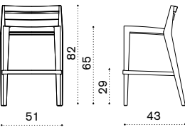
Counter stool h82 RBSGH1T1 cushion RBCUSGA___
